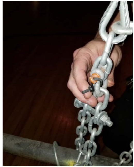
3 EXAMPLES: IMPROPER TRIM CHAINS
