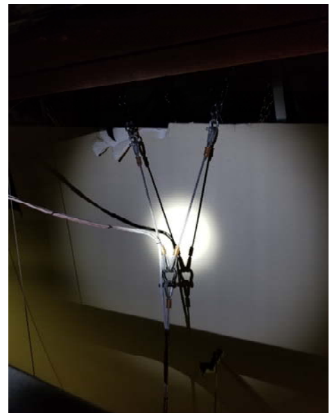
SPEAKER CLUSTER SHACKLES NOT MOUSED
