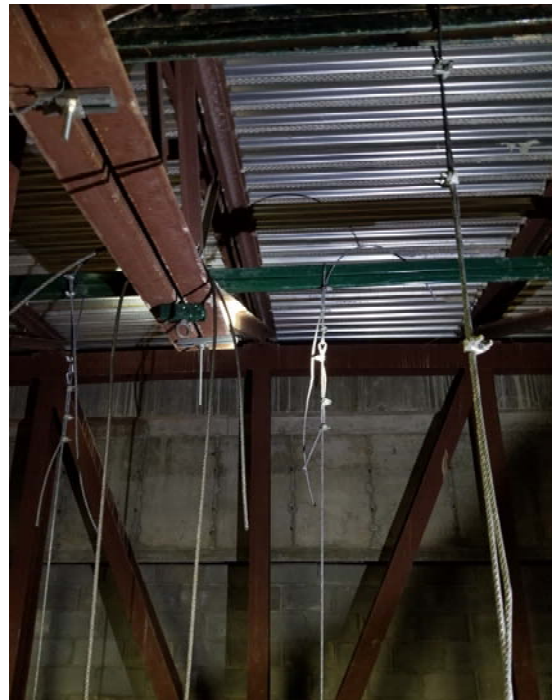
BARE WIRE WRAPS, IMPROPER TERMINATIONS, MESSY APPLICATION OF RIGGING TECHNIQUES
